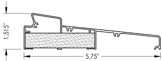
18 INSWING THRESHOLD
