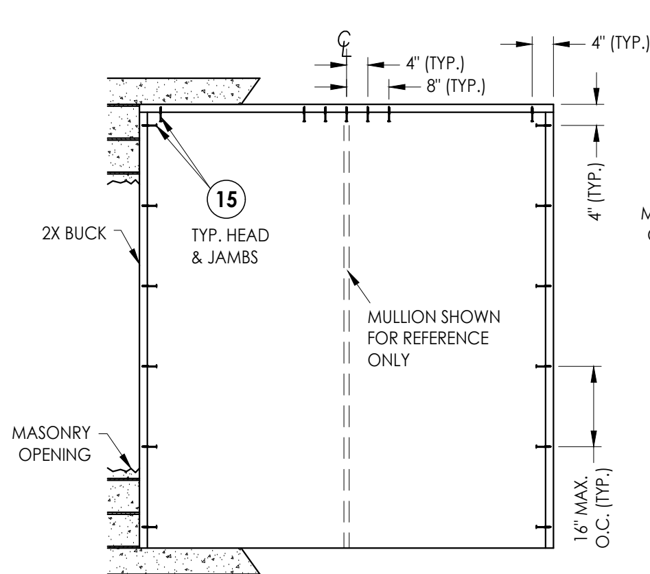
BUCK ANCHORING
