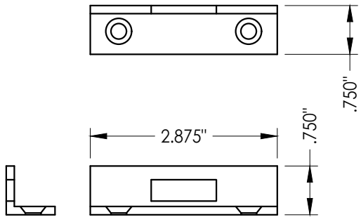
63 SURFACE BOLT STRIKE PLATE
