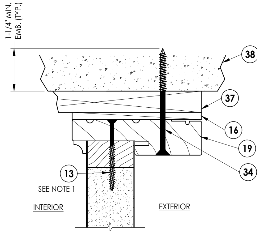
3 5 VERTICAL CROSS SECTION SHOWN w/ 1X SUB-BUCK
