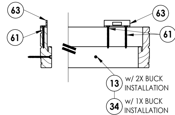
DETAIL "2" SURFACE BOLT @ HEAD
