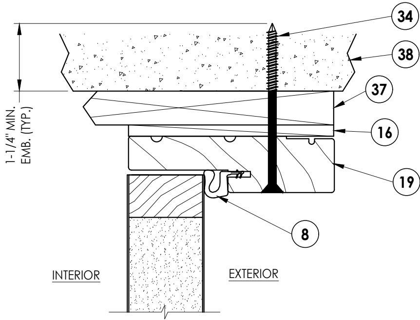
2 4 VERTICAL CROSS SECTION SHOWN w/ 1X SUB-BUCK
