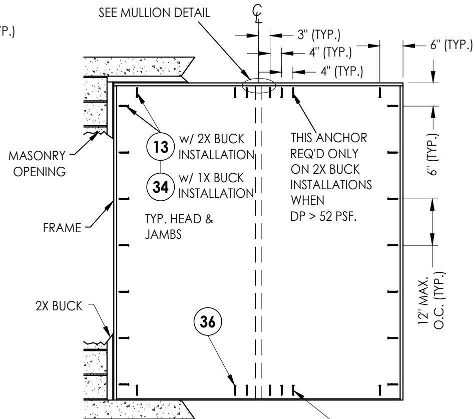
FRAME ANCHORING
