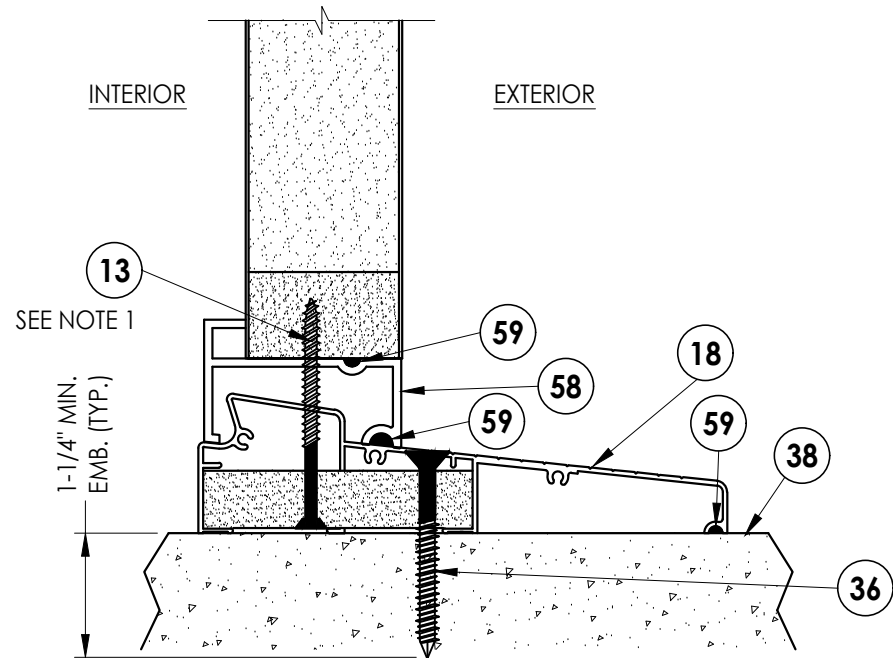
1 5 VERTICAL CROSS SECTION
